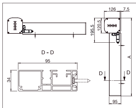
Wall installation with clips A = Total height
