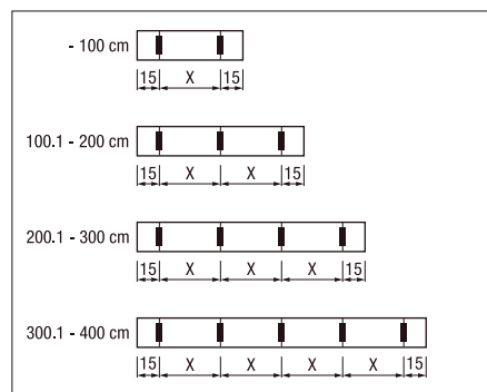
Arrangement and number of mounting brackets/punches or clips
