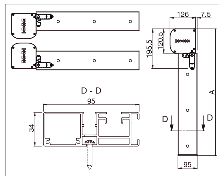
Soffit installation A = Total height
