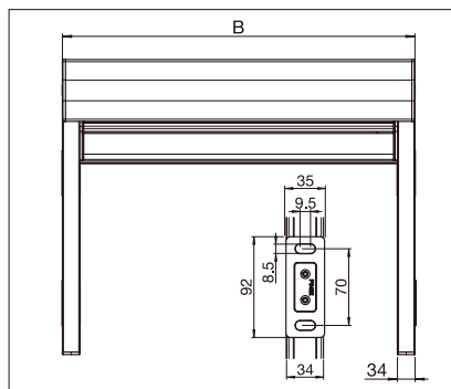
Wall installation B = Total width
