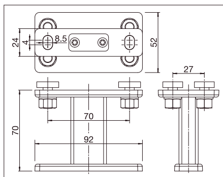
PS401/2 Soporte
