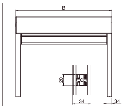
Bracket schedule with clips system B = Total width
