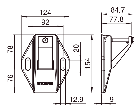
S821/1 Muro/soporte a techo
