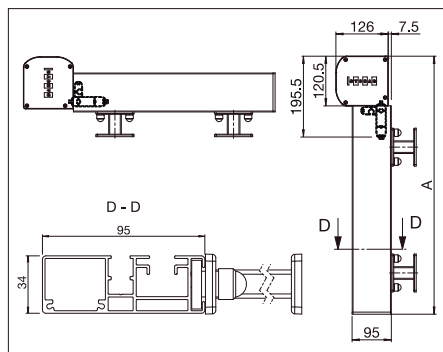
Wall installation A = Total height
