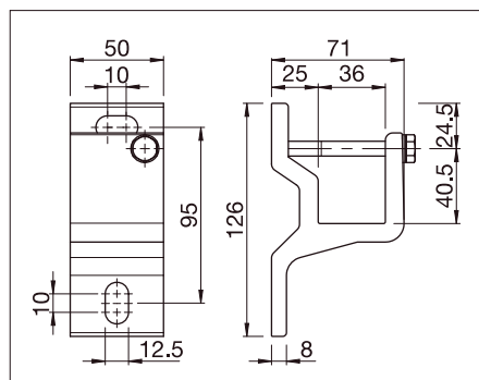
S221/5 Soporte
