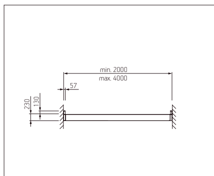
Vista frontal TR4520
